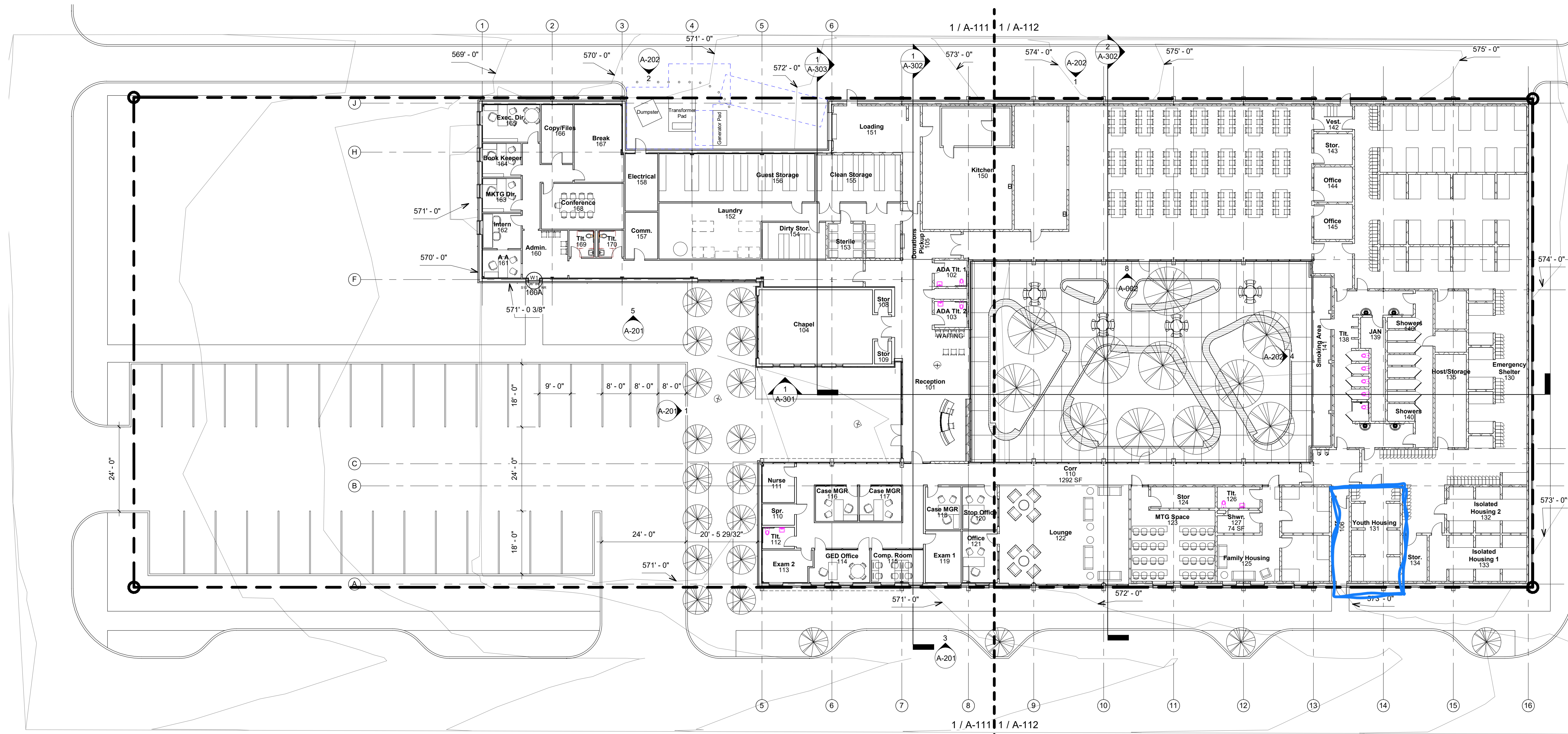
A7 Composite First Floor Plan Lvl 1 1/16" = 1'-0"
