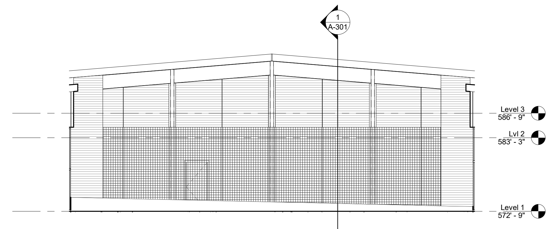
4 Courtyard West 1/8" = 1'-0"
