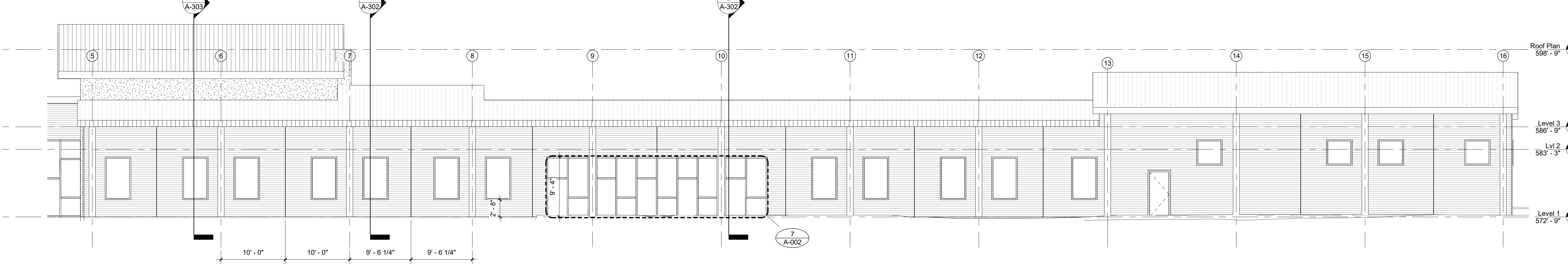
3 South Elevation 1/8" = 1'-0"
