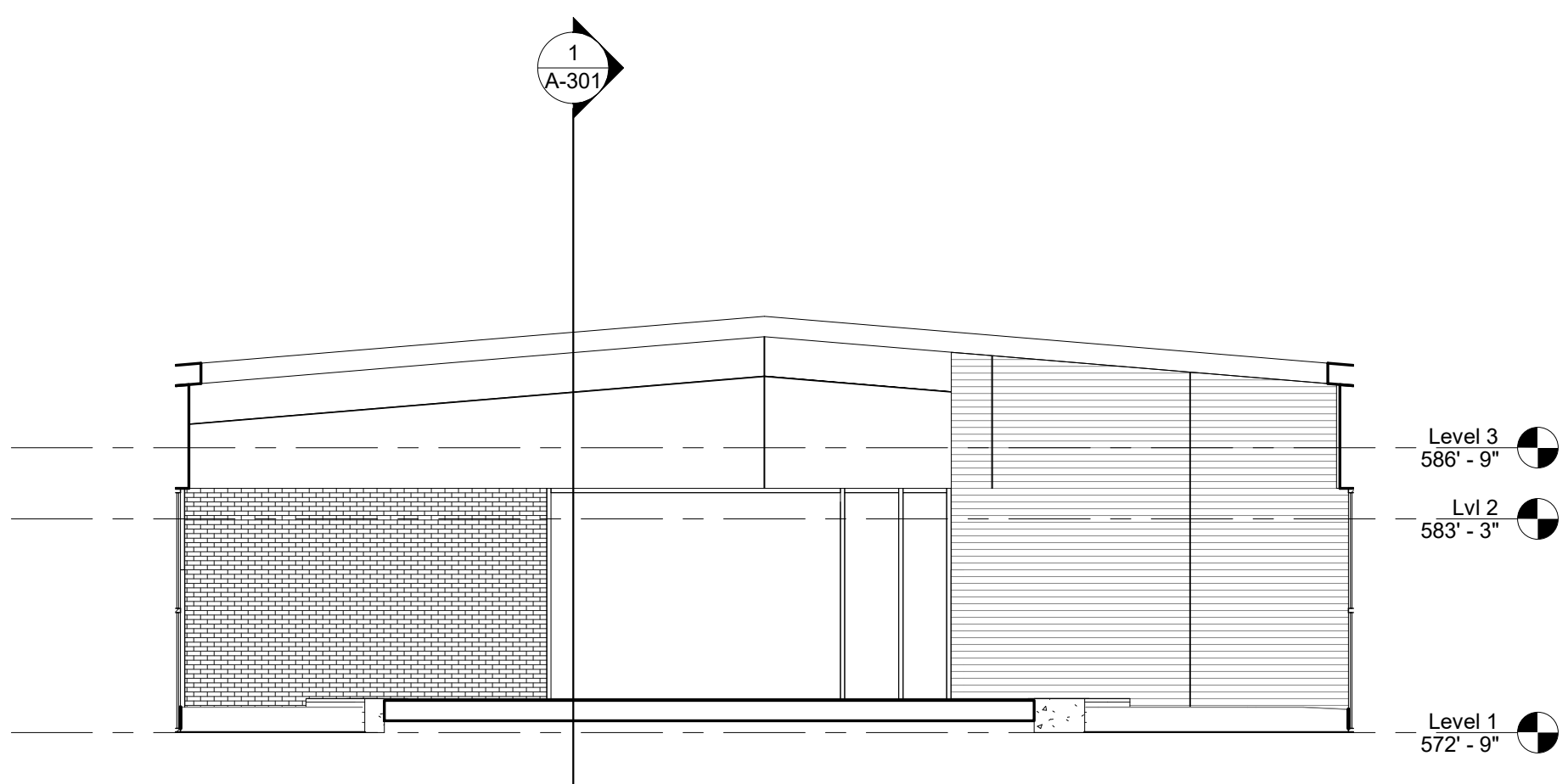
3 Courtyard East 1/8" = 1'-0"
